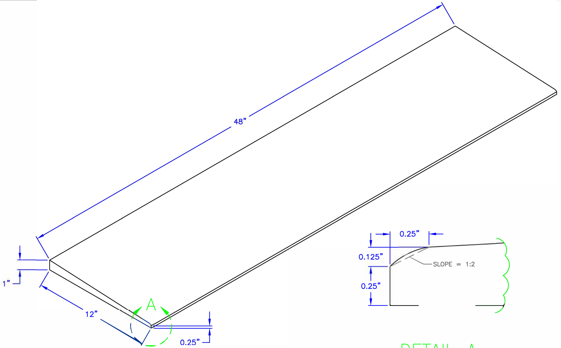
DETAIL A
